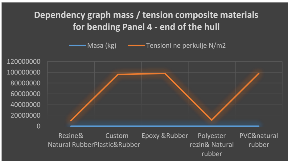
Fig NO 9 – Dependence / tension strain chart for composite materials Panel 4
