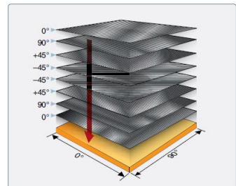
Figure 7-2. Quasi-isotropic material lay-up.
