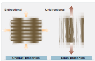
Figure 7-1. Bidirectional and unidirectional material properties.
