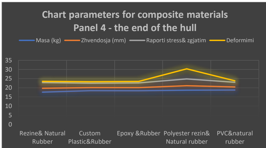
Fig No 10 - Chart parameters for composite materials Panel 4
