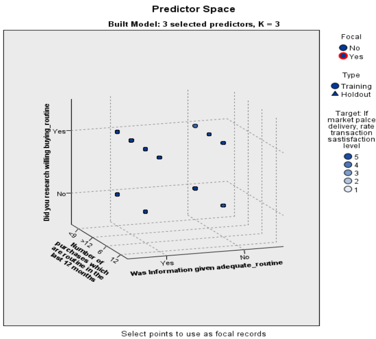
This chart is a lower-dimensional projection of the predictor space, which contains a total of 14 predictors.
