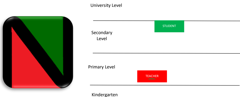
Figure 1: 'N' Theory
